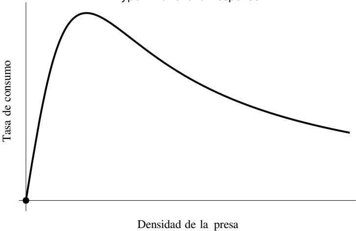
Type IV functional response
