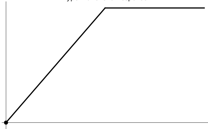
Type I functional response
