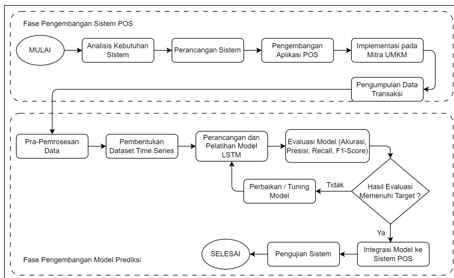
Gambar 3.1 Alur Penelitian
