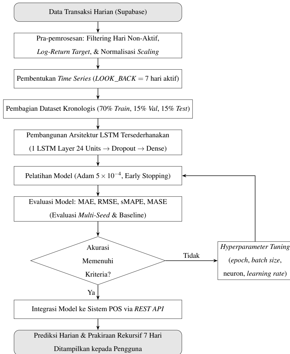
Gambar 3.18 Alur Kerja Algoritma Long Short-Term Memory (LSTM)
