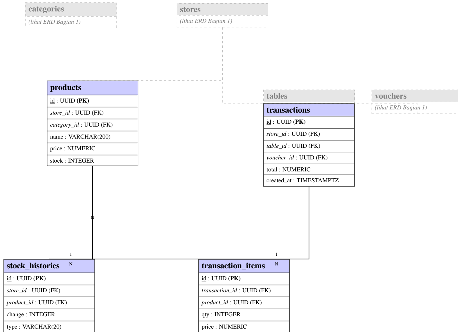
Gambar 3.7 Entity Relationship Diagram (ERD) Sistem POS — Bagian 2: Tabel Transaksi
