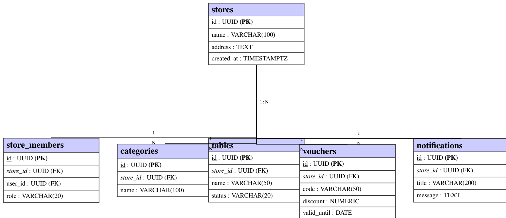
Gambar 3.6 Entity Relationship Diagram (ERD) Sistem POS — Bagian 1: Tabel Master
