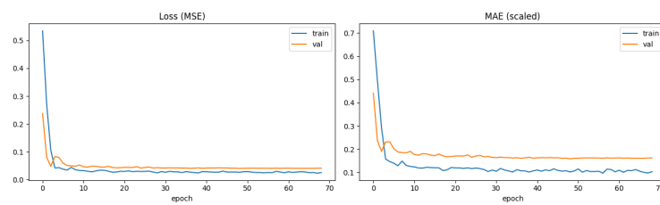
Gambar 4.1 Kurva Kerugian Pelatihan ( Training Loss Curve ) Model LSTM
