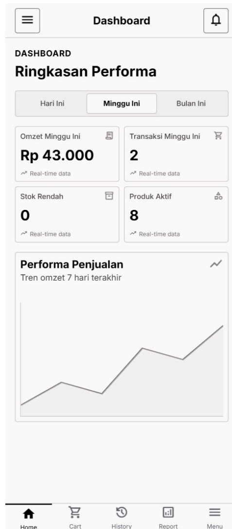
Gambar 3.15 Wireframe Halaman Dasbor Owner
