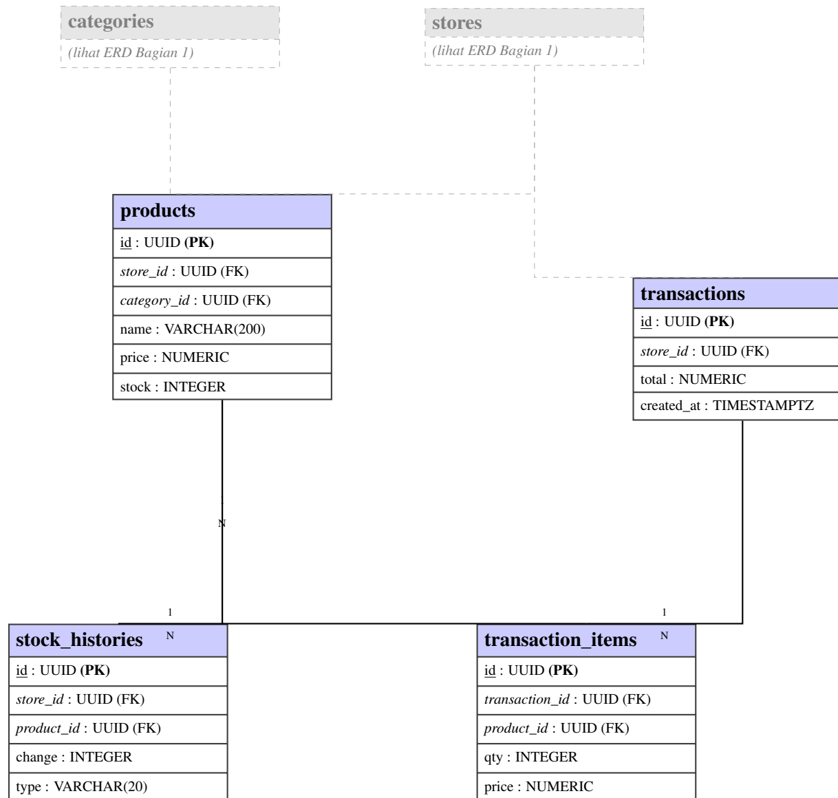
Gambar 3.4 Entity Relationship Diagram (ERD) Sistem POS — Bagian 2: Tabel Transaksi
