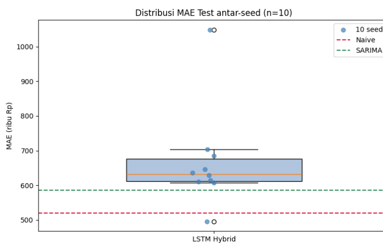
Gambar 4.3 Boxplot Distribusi MAE Hasil Pengujian Multi-Seed
