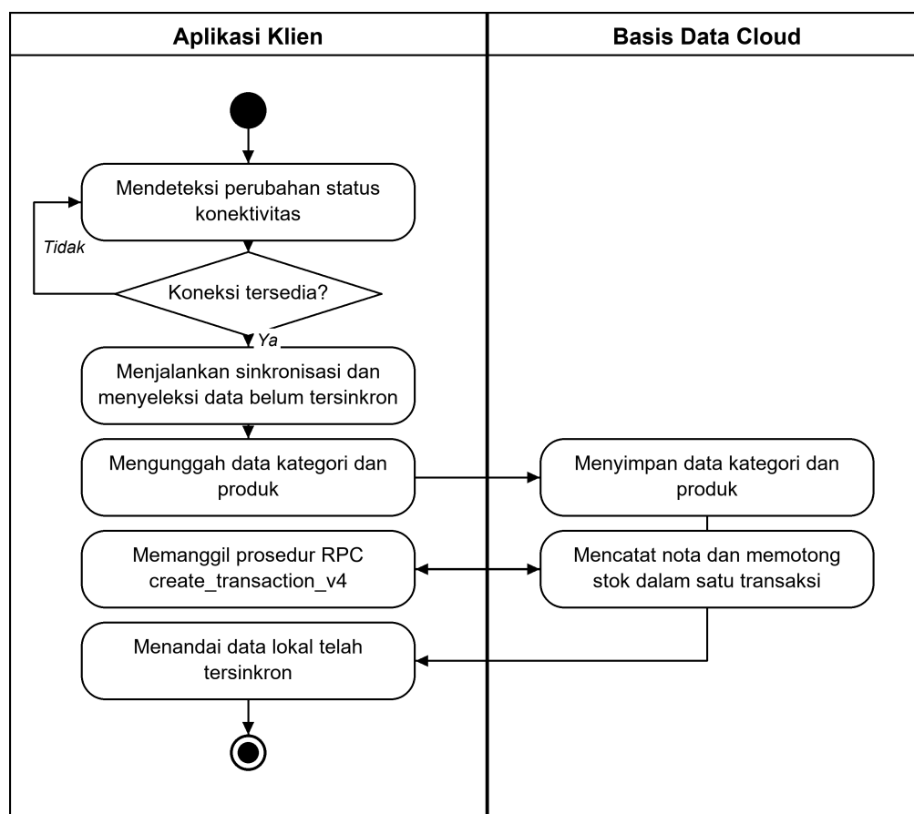
Gambar 3.6 Activity Diagram Sinkronisasi Data
