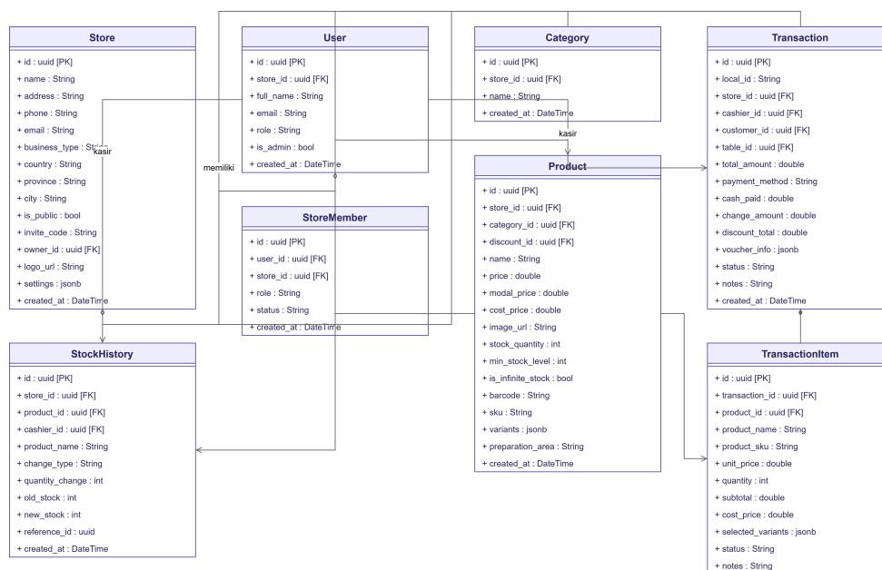
Gambar 3.16 Class Diagram Sistem POS
