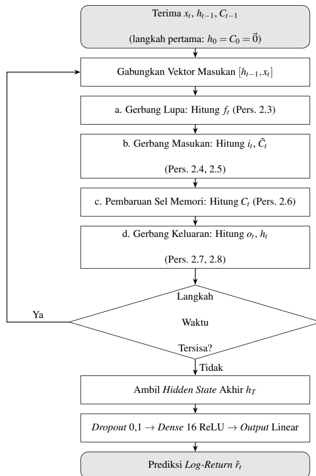
Gambar 3.31 Flowchart Perhitungan Sel Long Short-Term Memory
