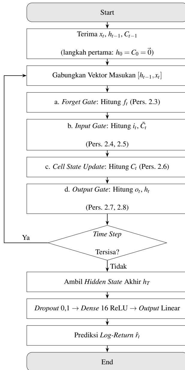
Gambar 3.31 Flowchart Perhitungan Sel Long Short-Term Memory
