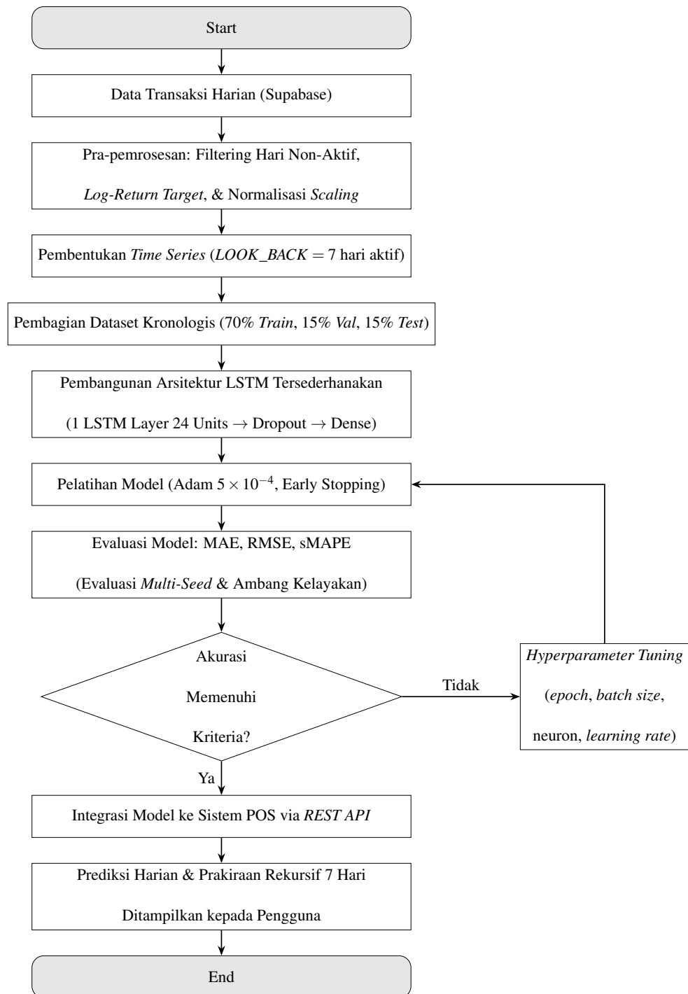
Gambar 3.30 Alur Kerja Algoritma Long Short-Term Memory (LSTM)
