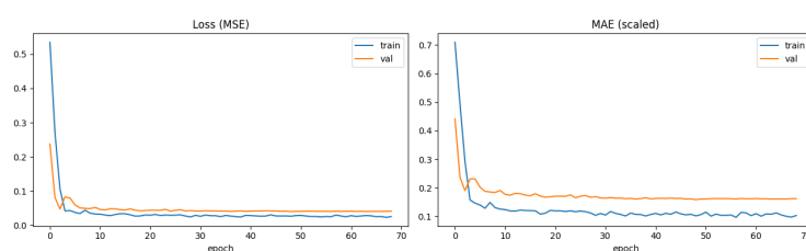
Gambar 4.20 Kurva Kerugian Pelatihan ( Training Loss Curve ) Model LSTM
