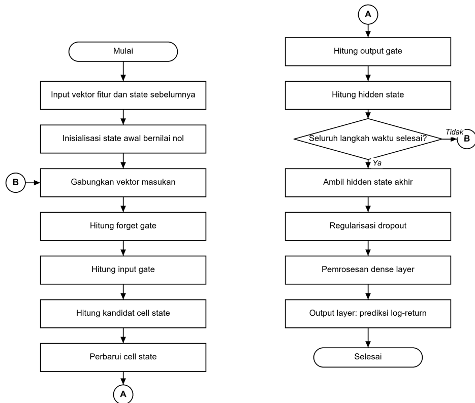
Gambar 3.31 Flowchart Perhitungan Sel Long Short-Term Memory
