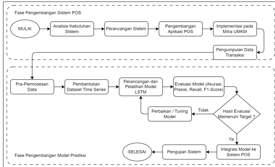
Gambar 3.17 Alur Penelitian
