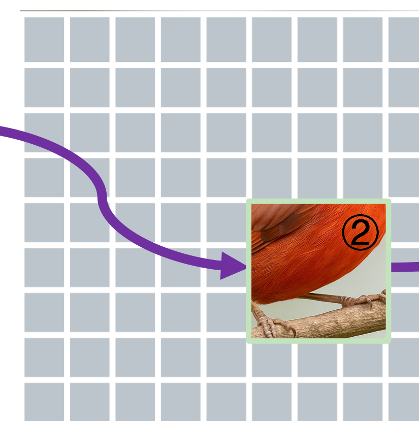
Sequential Prediction
