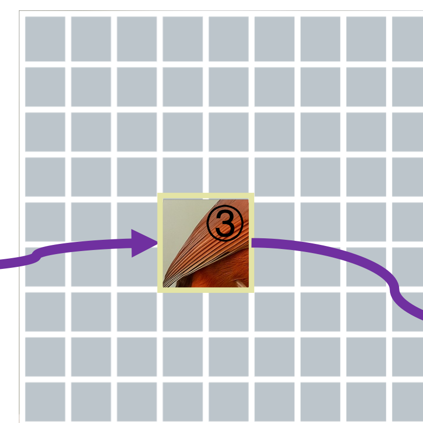
Sequential Prediction
