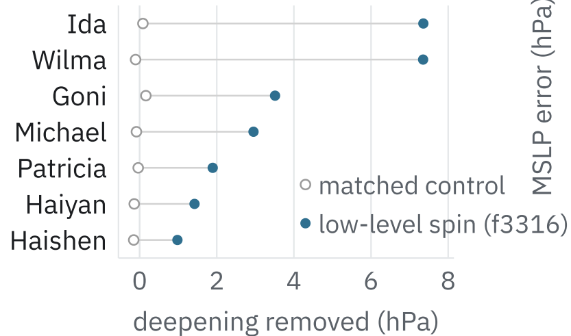
a Effect of low-level spin ablation across storms
