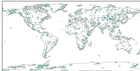
f3404 — its matched control
