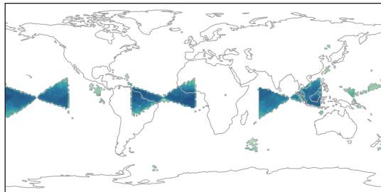
f2075 — bowties
