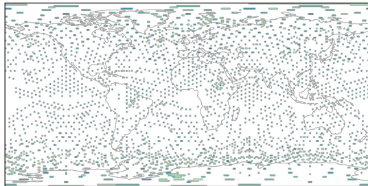
f2954 — full lattice
