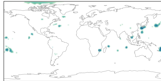
f3243 — tropical cyclone
