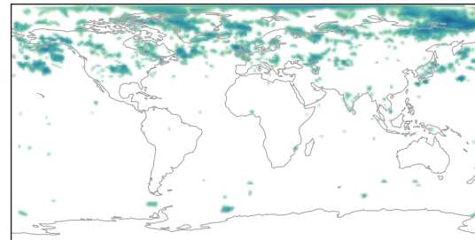
f3861 — low-level vorticity
