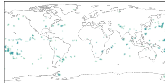
f2401 — convection
