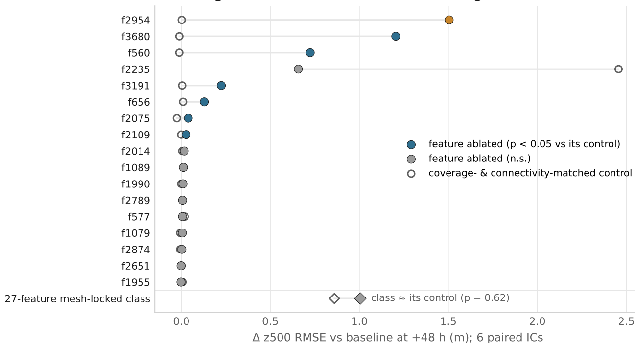
e One grid-locked feature is load-bearing; the class is not
