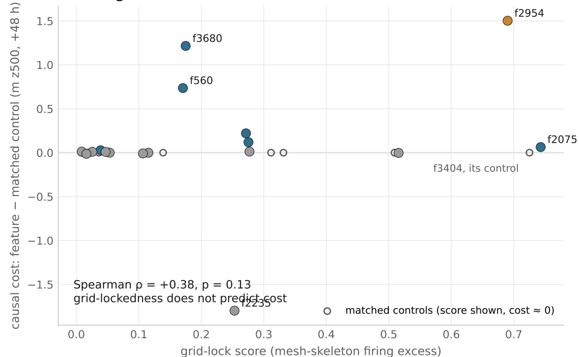
f Being mesh-locked is not what makes a feature matter
