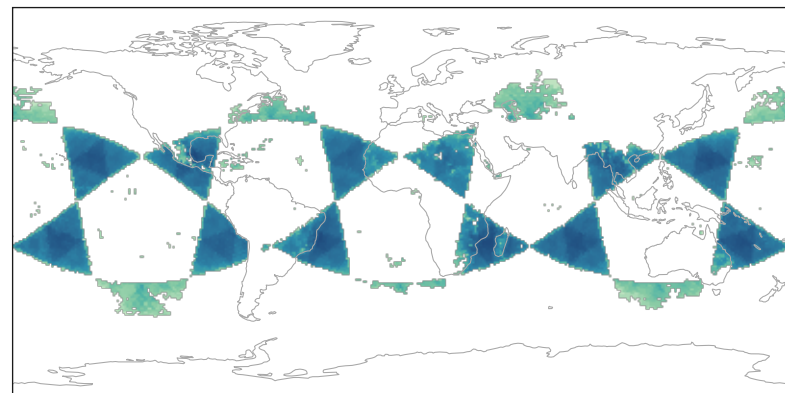
Feature 2585
