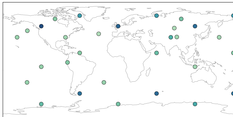
Feature 2989
