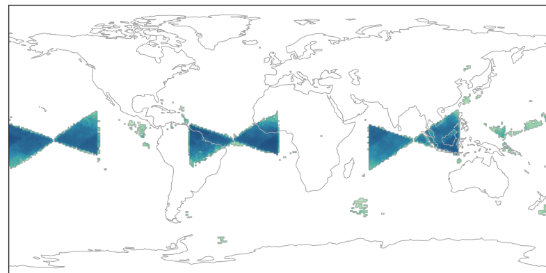
Feature 2075
