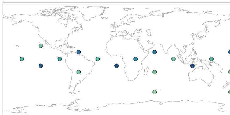
Feature 407
