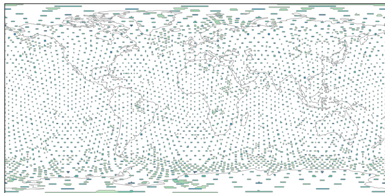
Feature 2954
