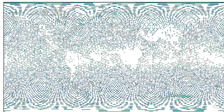
Feature 3535
