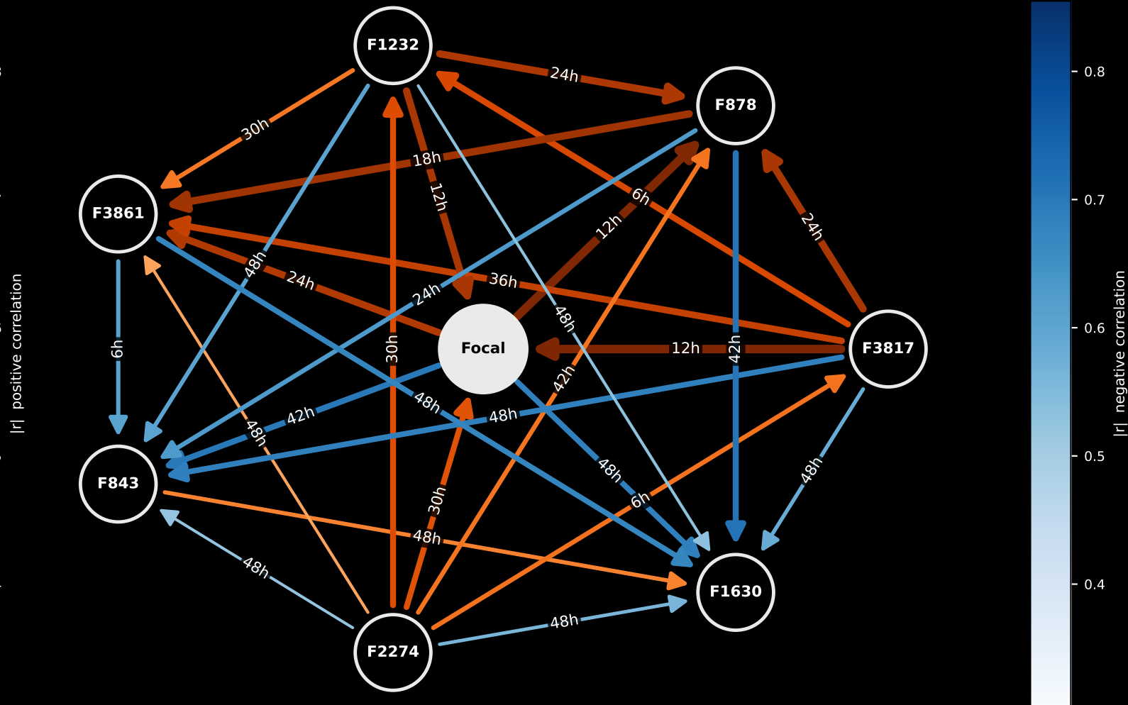
ncy Graph for Tropical Cyclone / Hurricane (threshold |r| \geq 0.3 , \tau_{\max} = 48\text{h} )
