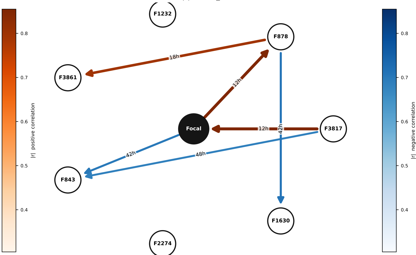
Lagged Dependency Graph for Tropical Cyclone / Hurricane Tracker (threshold |r| \geq 0.3 , \tau_{\max} = 48h )
