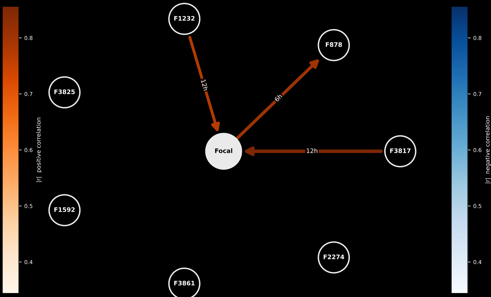
Lagged Dependency Graph for Tropical Cyclone / Hurricane Tracker (threshold |r| \geq 0.3 , \tau_{\max} = 48\text{h} )
