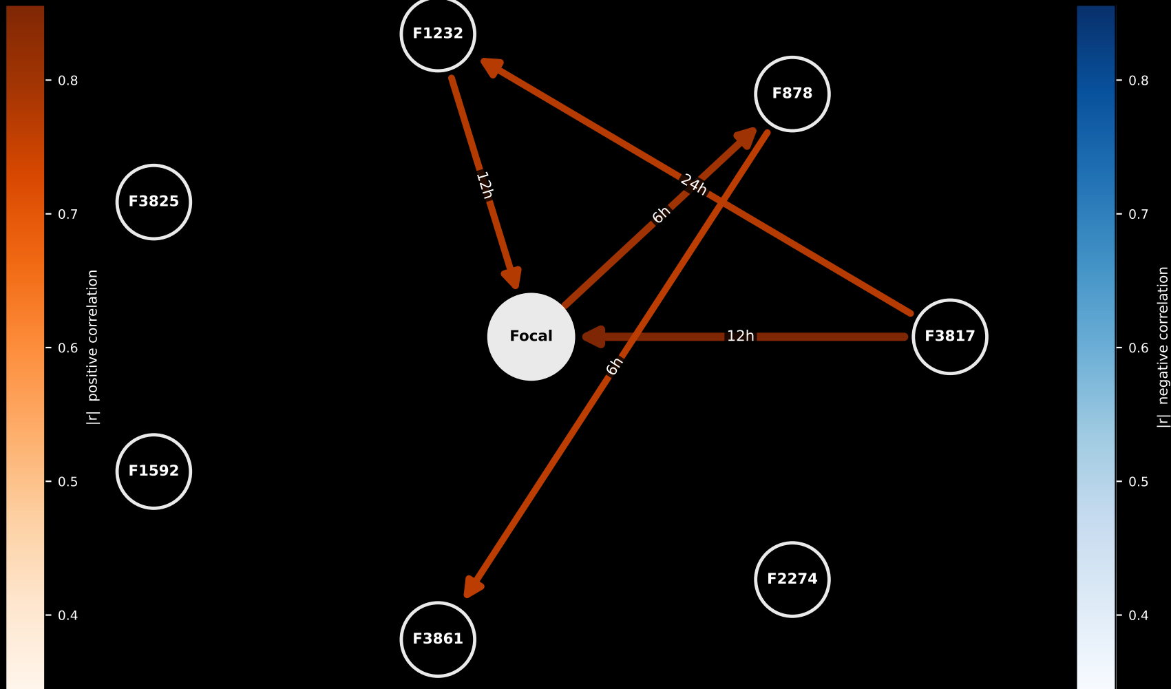
Lagged Dependency Graph for Tropical Cyclone / Hurricane Tracker (threshold |r| \geq 0.3 , \tau_{\max} = 48\text{h} )
