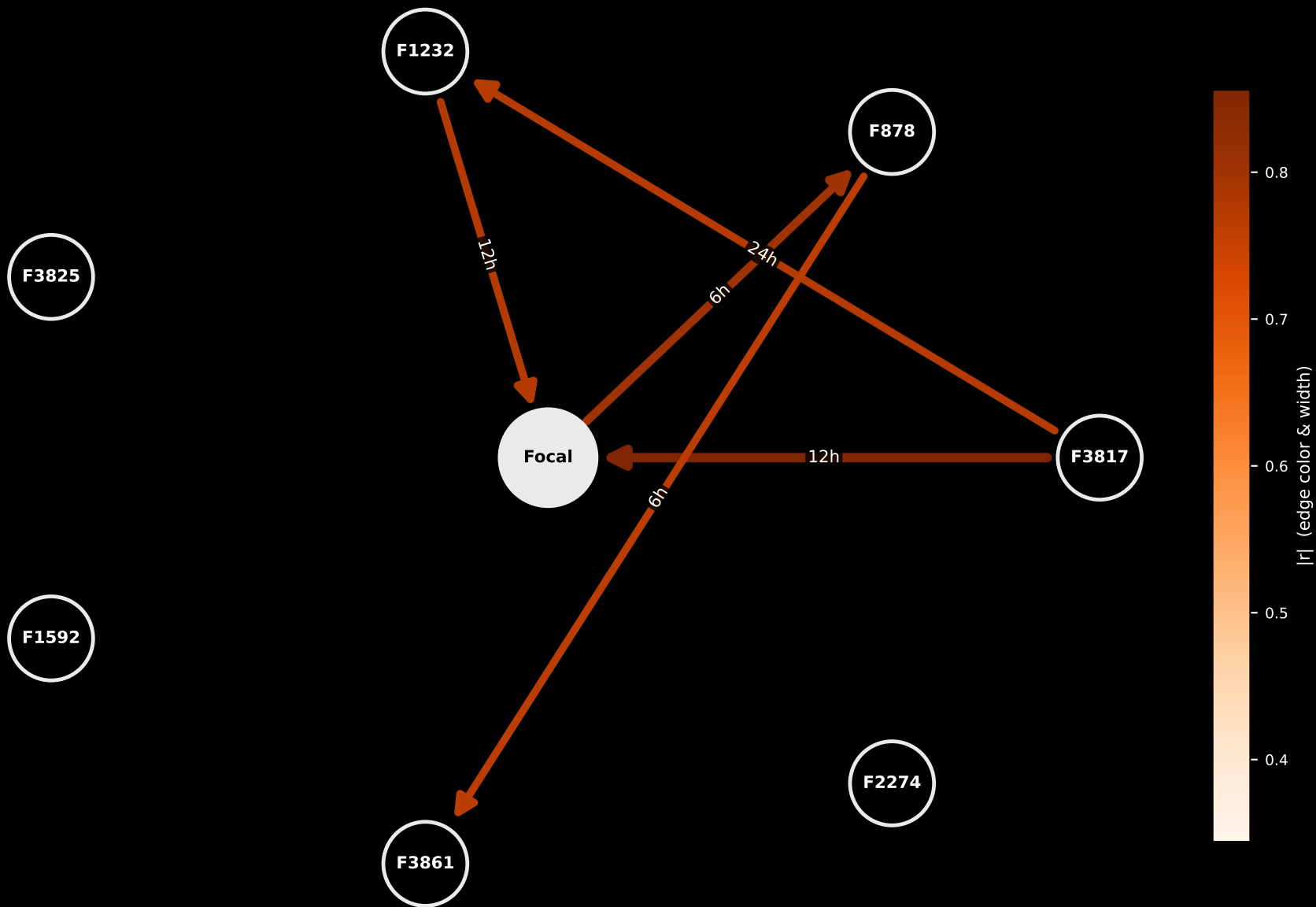
Lagged Dependency Graph for Tropical Cyclone / Hurricane Tracker (top 5 edges |r| \geq 0.3 , \tau_{\max} = 48h )
