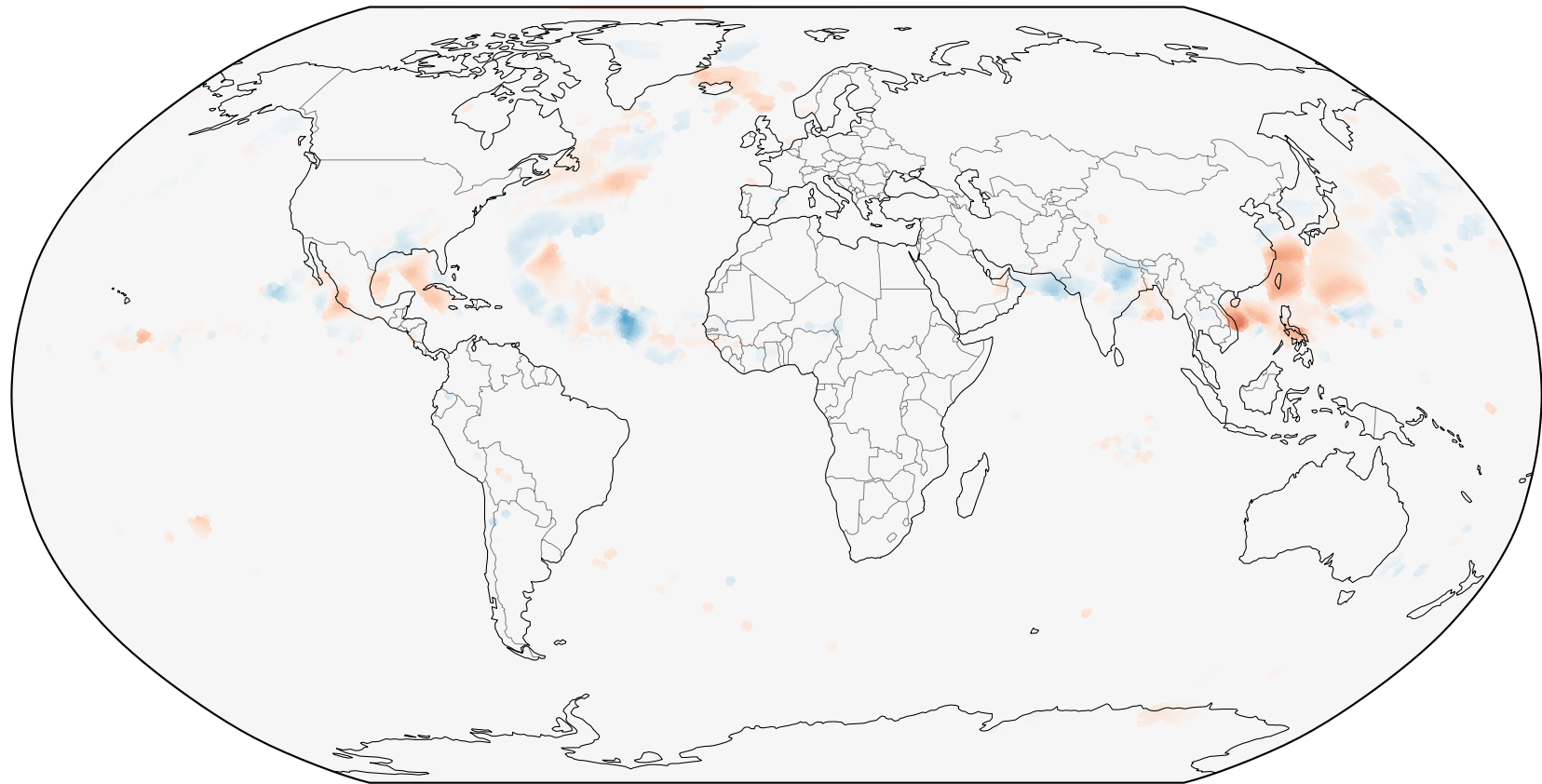
Feature 3243 x T 300 hPa [T=168 timesteps, log1p activations]
