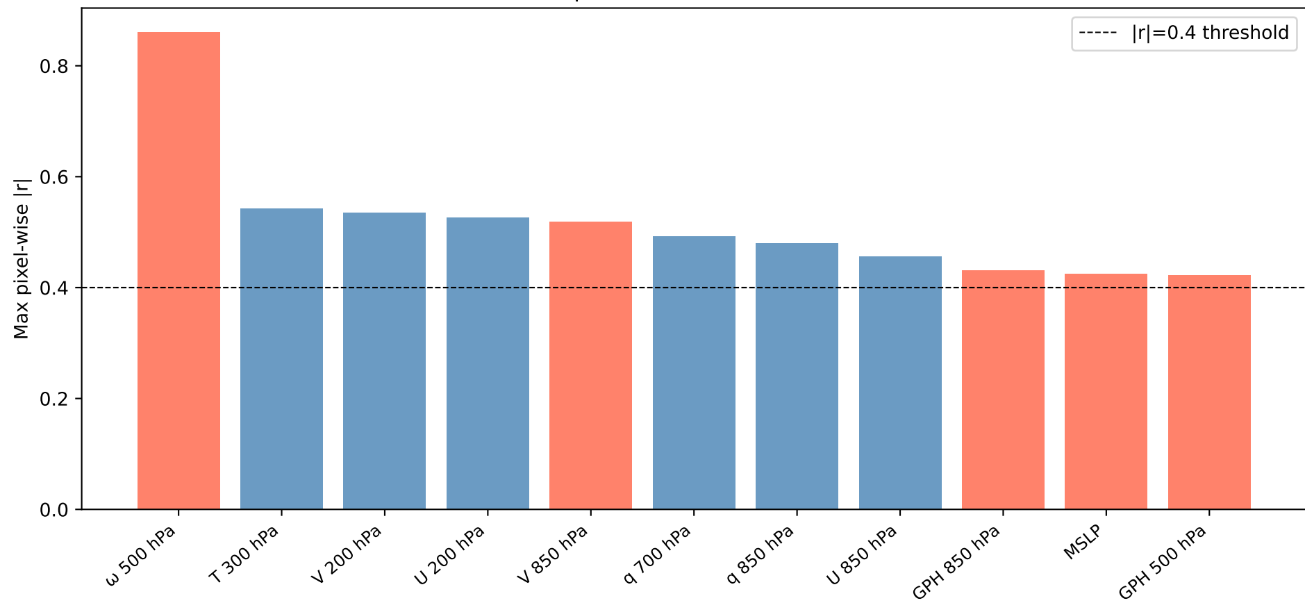
Feature 3243: Peak spatial correlation with ERA5 fields (T=168)
