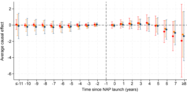
AMU score event-study estimates
