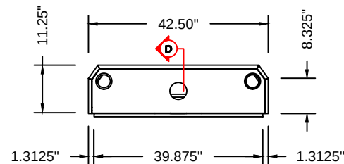
Plan View SCALE: 3/8" = 1'-0"
