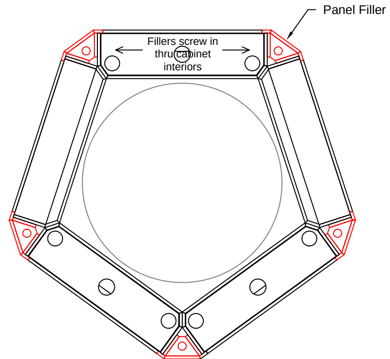
Typical Column Surround SCALE: 1/2" = 1'-0"
