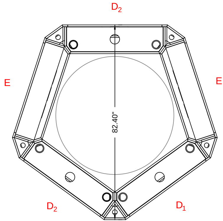
Column Plan View SCALE: 1/2" = 1'-0"
