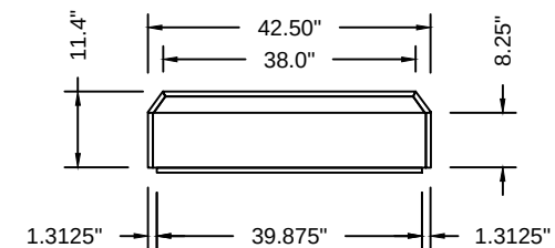
Plan View SCALE: 3/8" = 1'-0"
