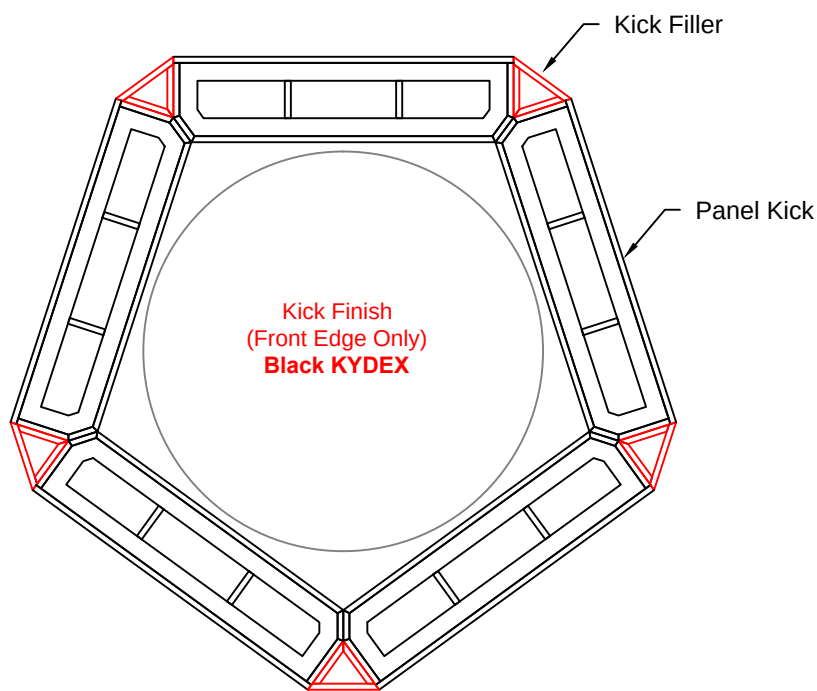
Typical Column Surround SCALE: 1/2" = 1'-0"
