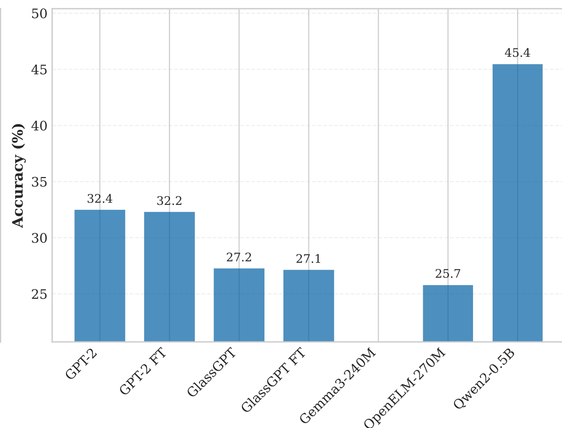
BoolQ Benchmark
