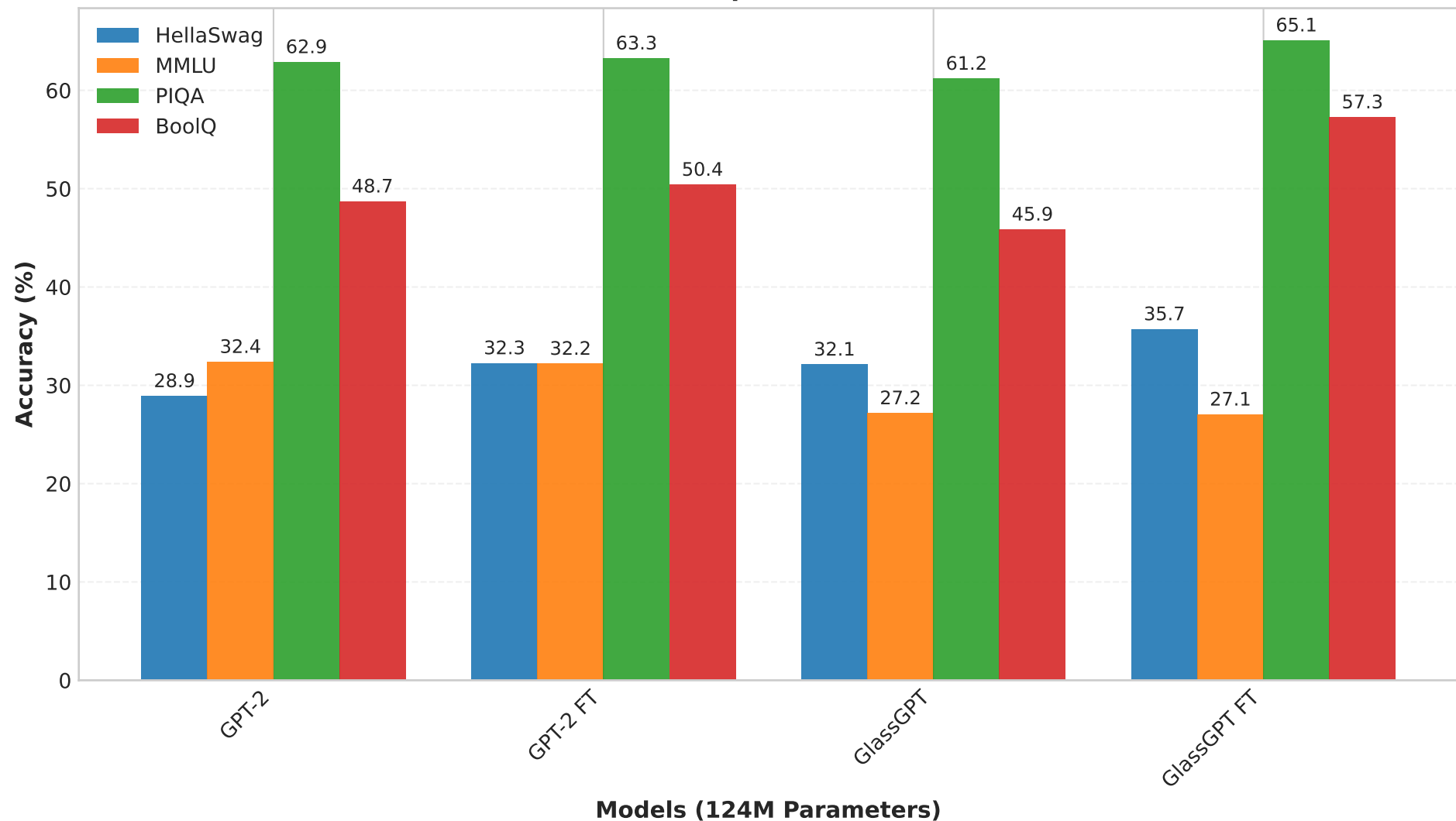
Benchmark Performance Comparison of 124M Parameter Models
