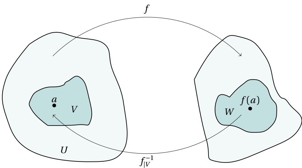
FIGURE 21 : Inversion locale.
