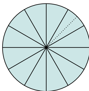
Disque \mathcal{D}
