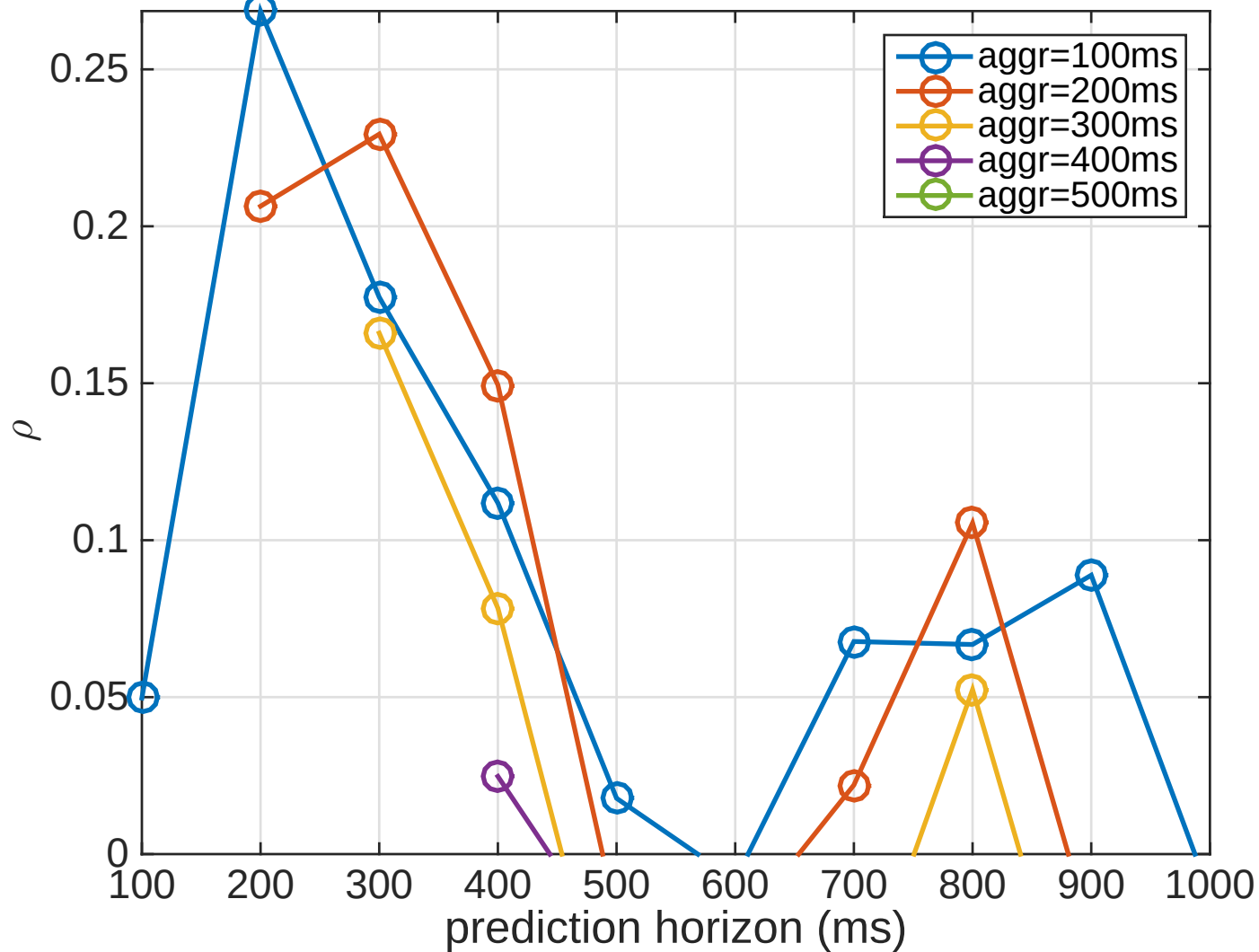
\rho above Baseline AR NN
