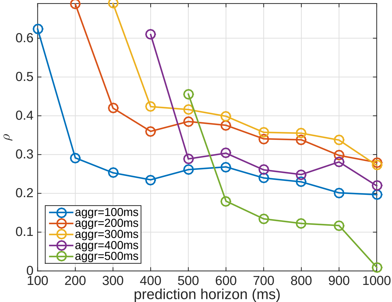
\rho SVM gaussian
