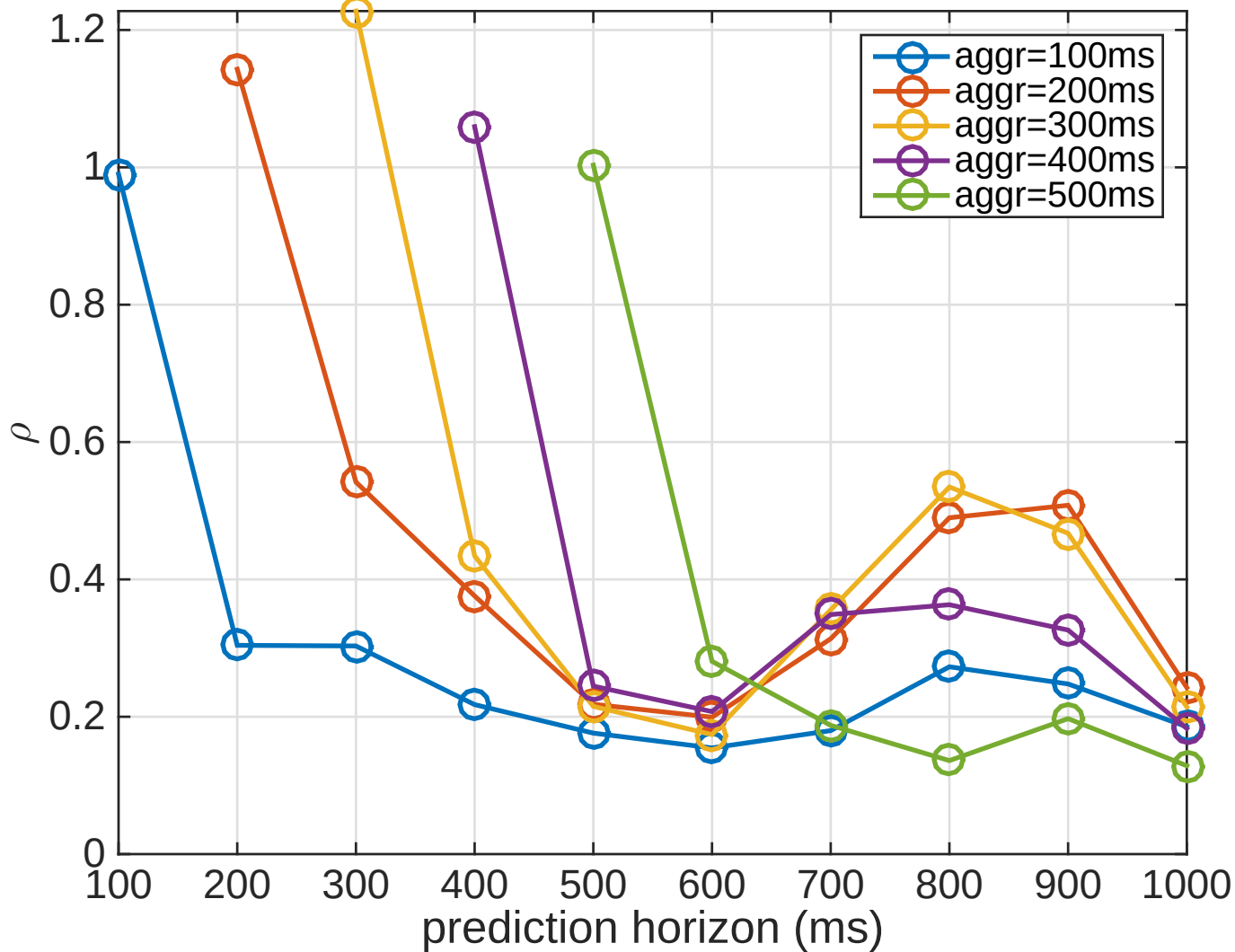
\rho above Baseline SVM poly
