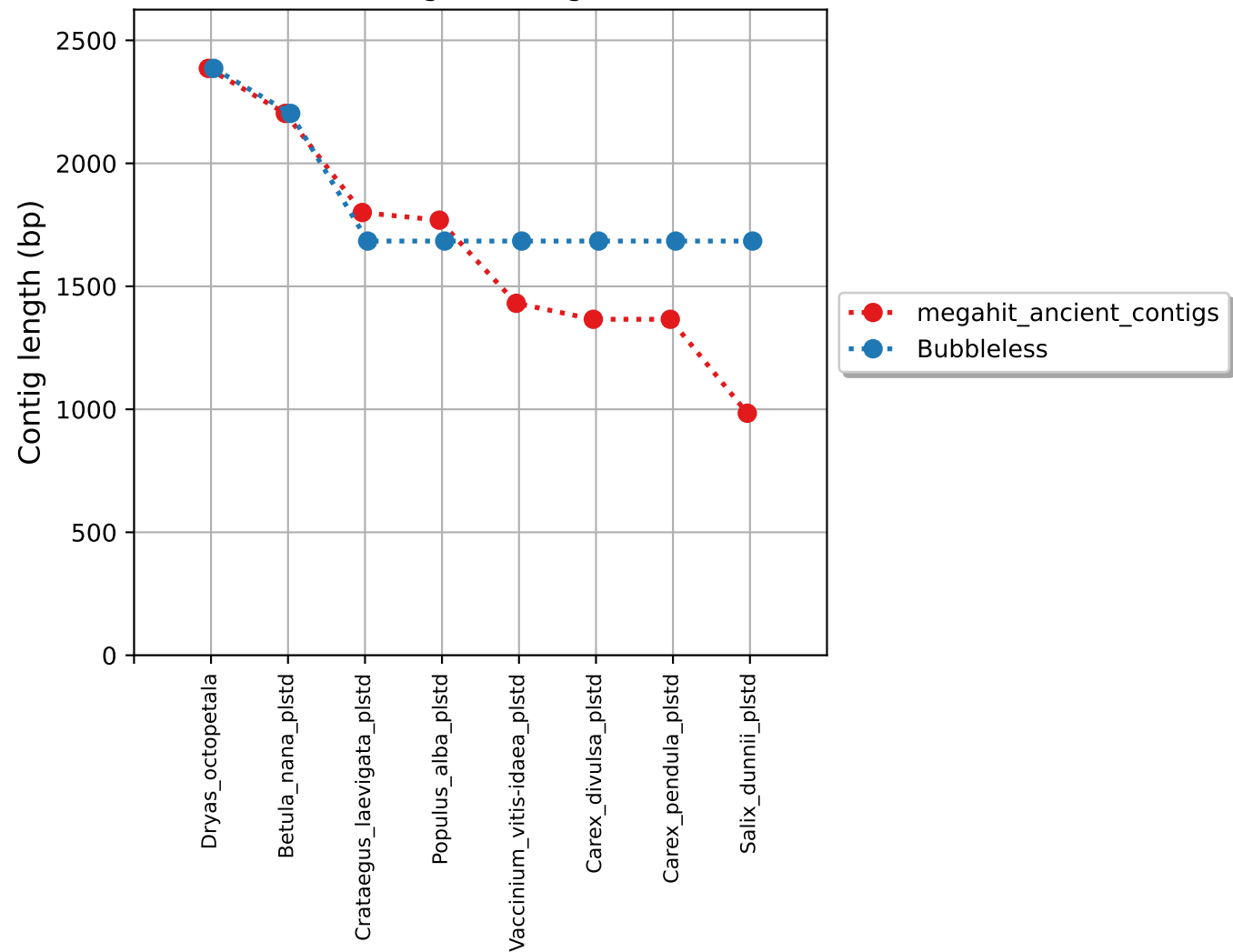
Largest contig
