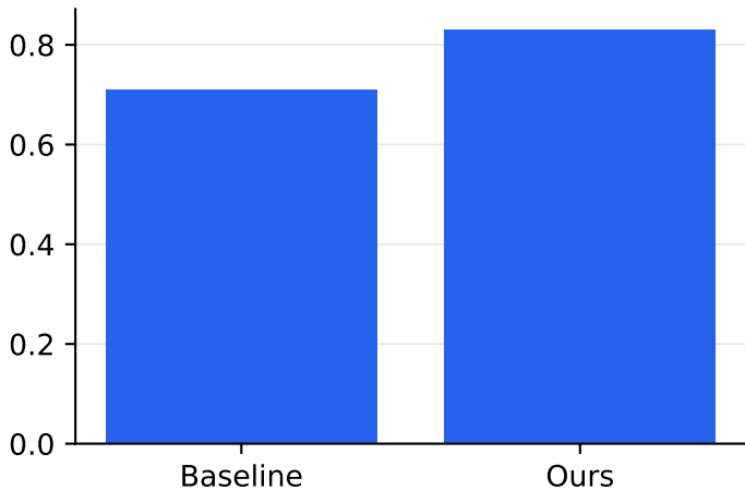
Benchmark Accuracy
