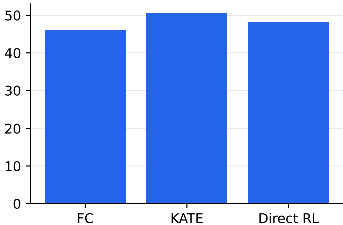
BFCL-V3 Average: KATE ablation
