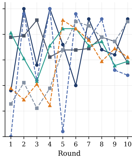
Recall
