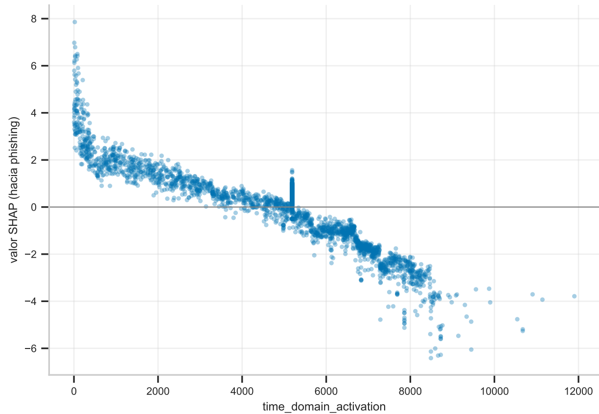
Dependencia SHAP: time_domain_activation
