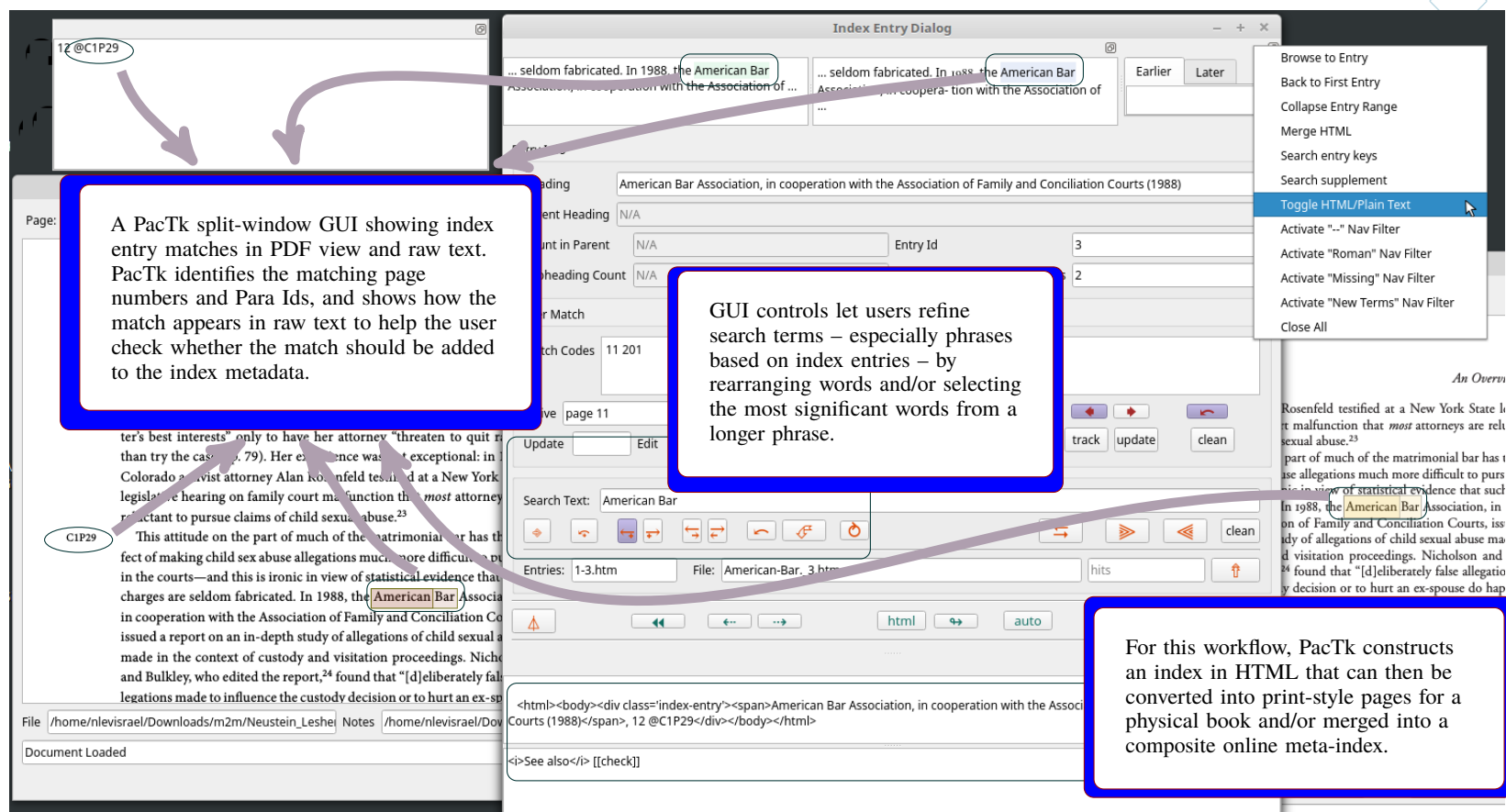
Figure 1: GUI functionality for compiling and curating indexes
