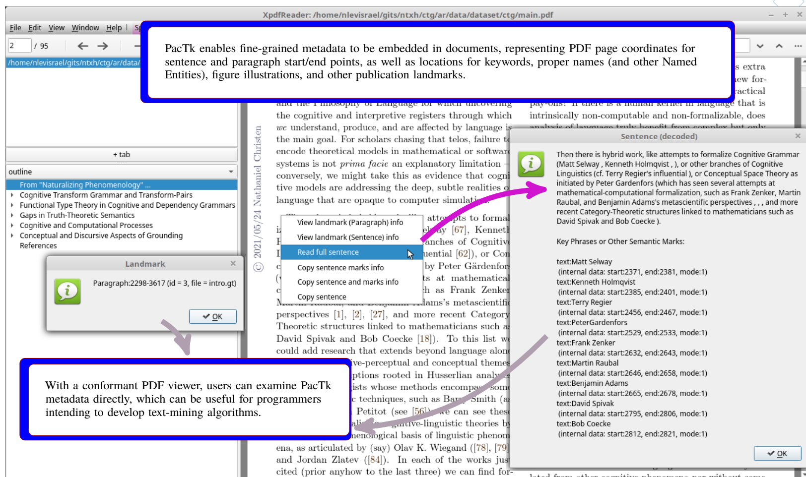
Figure 2: Enhanced GUI capabilities enabled by machine-readable text encoding
