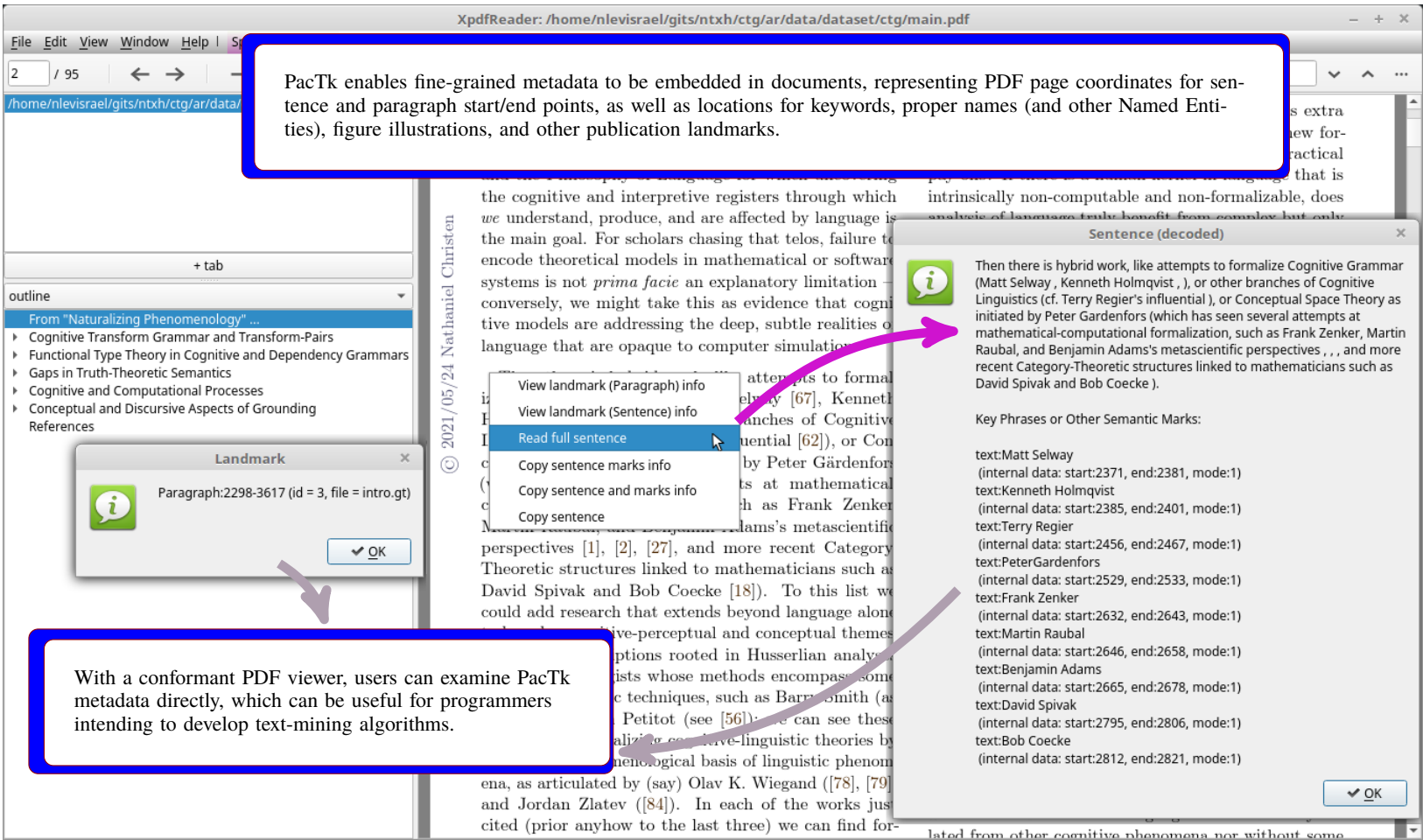
Figure 8: Enhanced GUI capabilities enabled by machine-readable text encoding
