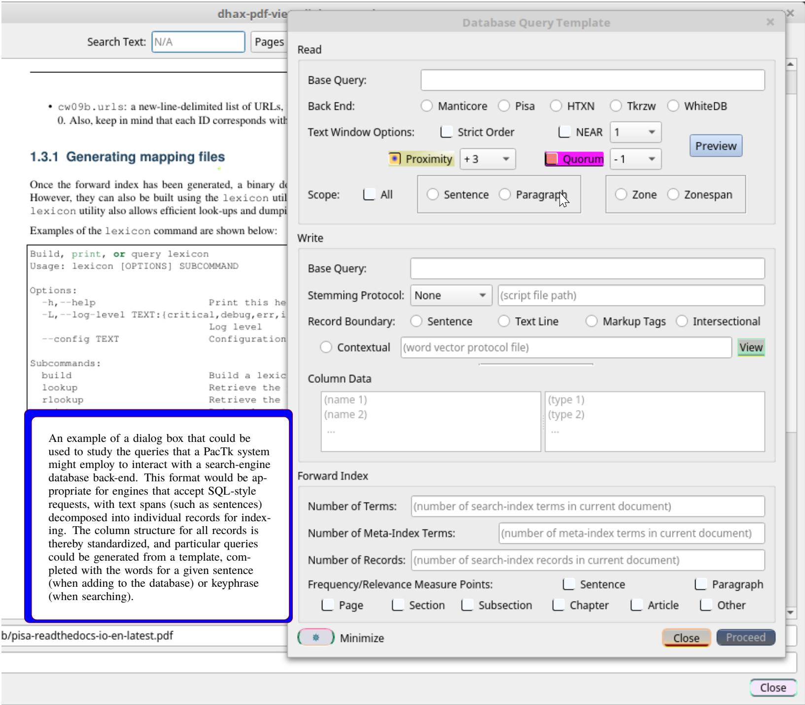
Figure 9: Configuring Default Back-End Queries
