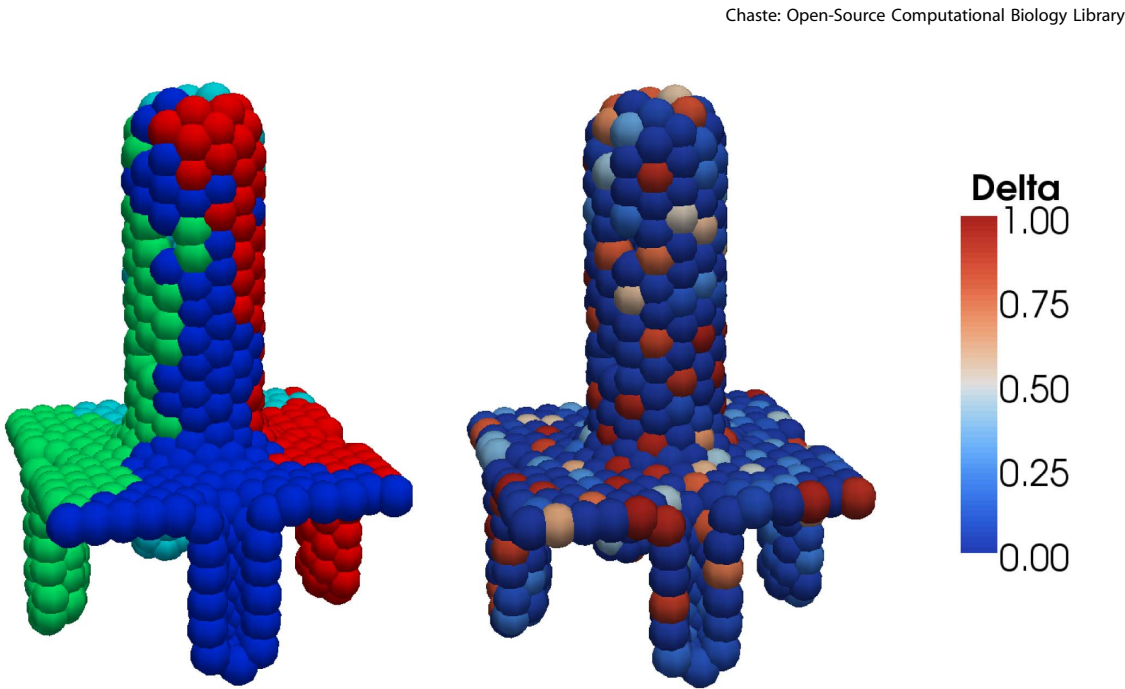
Figure 2. 3D off-lattice simulation confined to a 2D surface: small intestinal crypts and villus. Left: cells are labelled according to their ancestor cell; each crypt gives rise to a monoclonal population, with a multiclonal villus comprised of cells from each crypt. Right: the same simulation, here with cells labelled according to Delta levels (non-dimensionalised); Delta-Notch patterning occurs due to a signalling model inside each cell, which depends on the activity of neighbouring cells, and is thought to lead to differentiation into secretory and absorptive cell types. See also Video S2. doi:10.1371/journal.pcbi.1002970.g002
