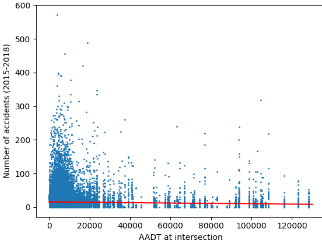
Figure 2: Average daily traffic flow (AADT) plotted against number_of_accidents.
