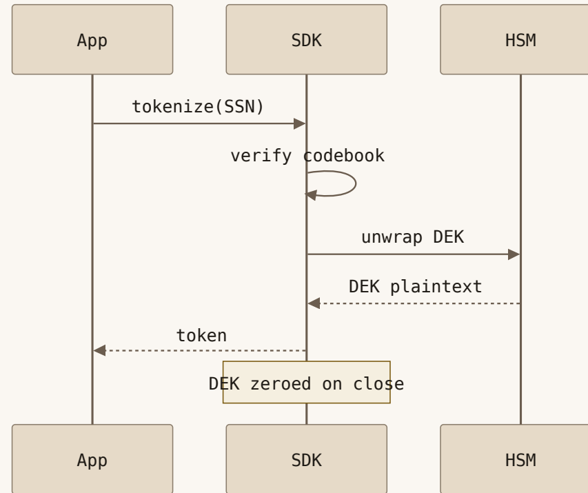
Tokenize call sequence
