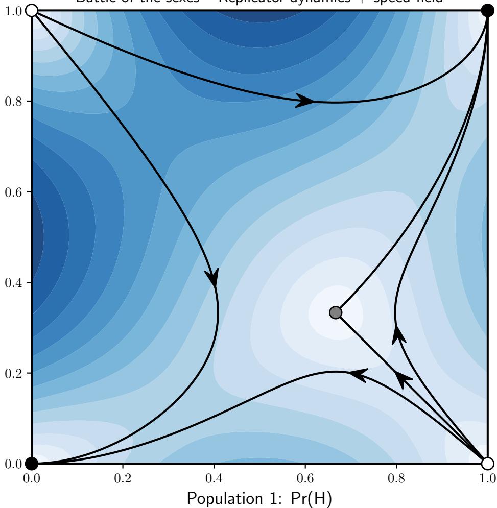
Battle of the sexes – Replicator dynamics + speed field
