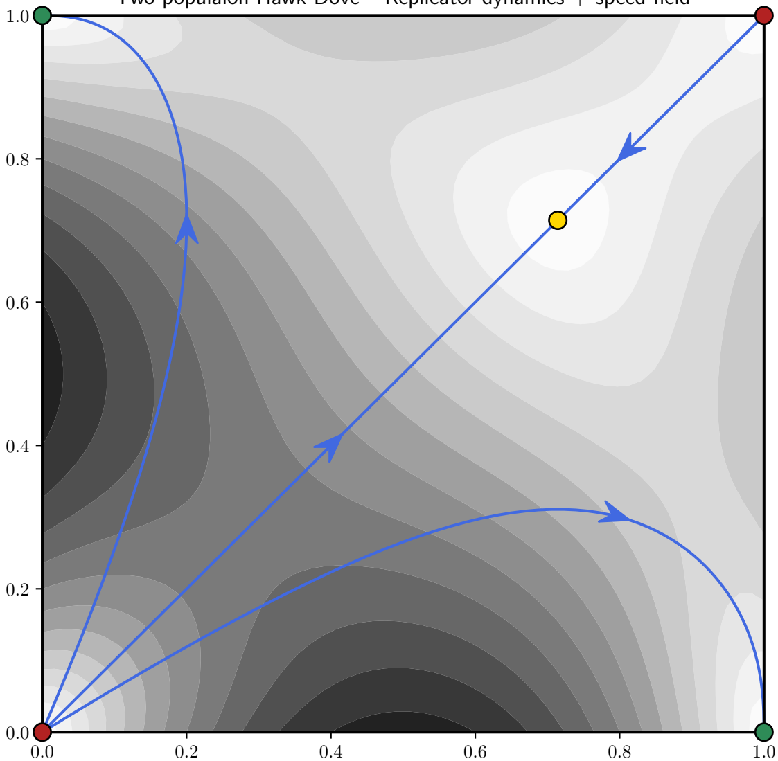
Two-population Hawk-Dove – Replicator dynamics + speed field
