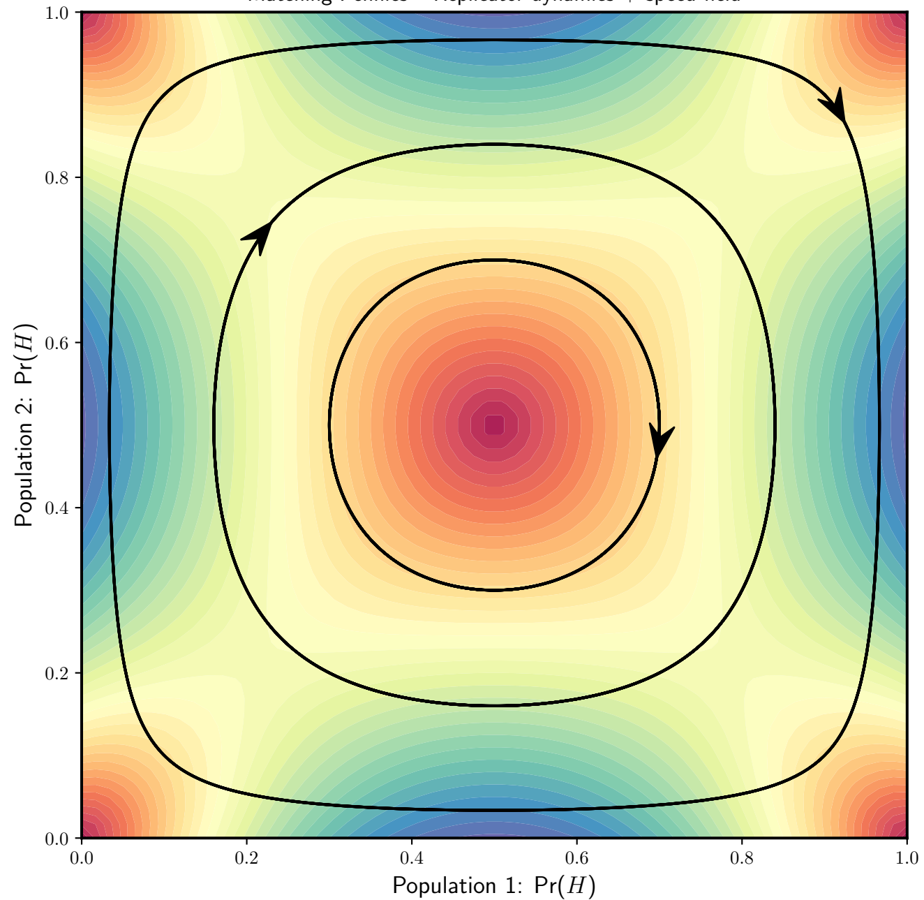
Matching Pennies – Replicator dynamics + speed field
