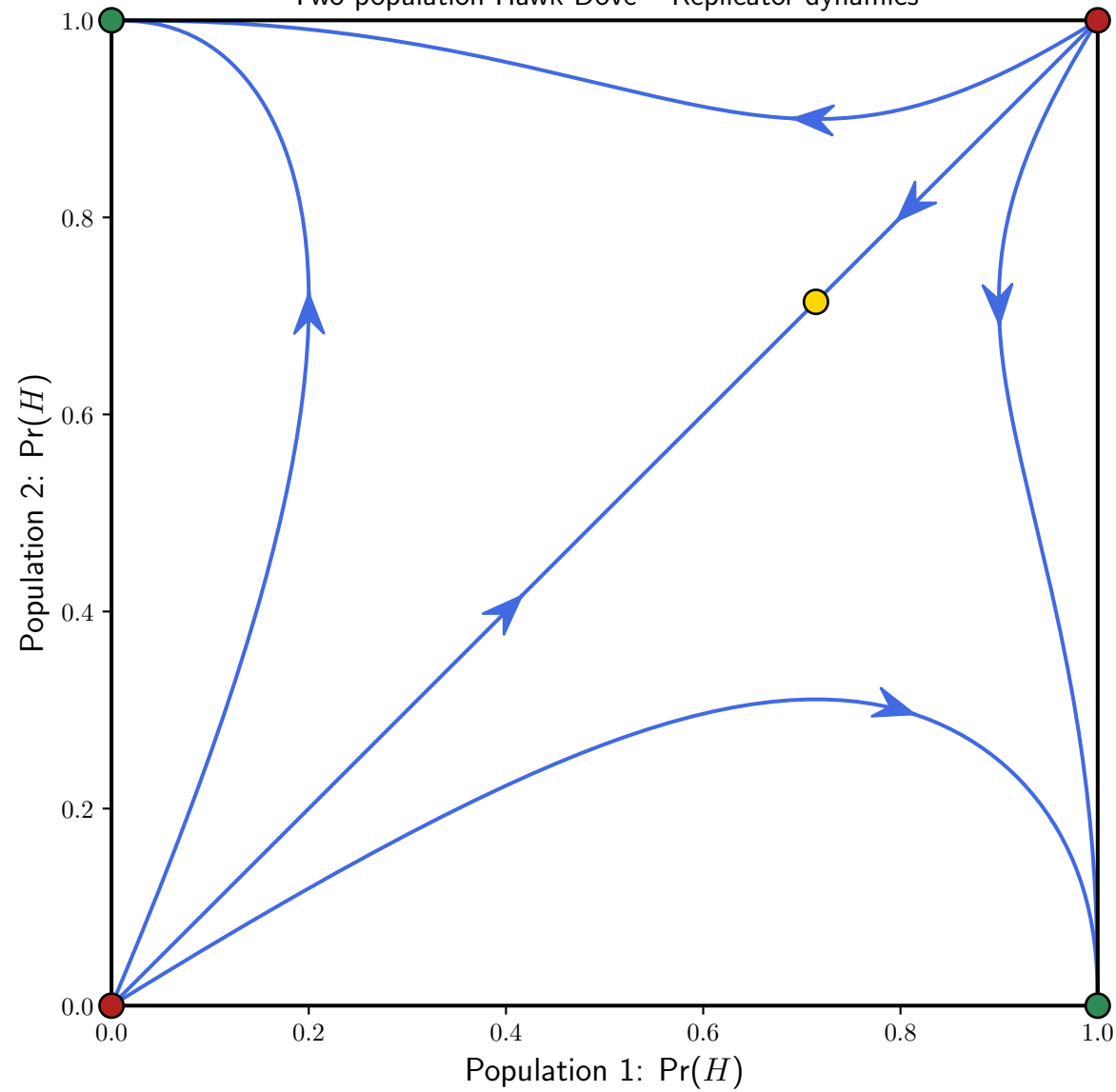
Two-population Hawk-Dove – Replicator dynamics
