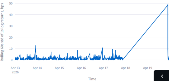
Local 60-Second Futures Volatility
